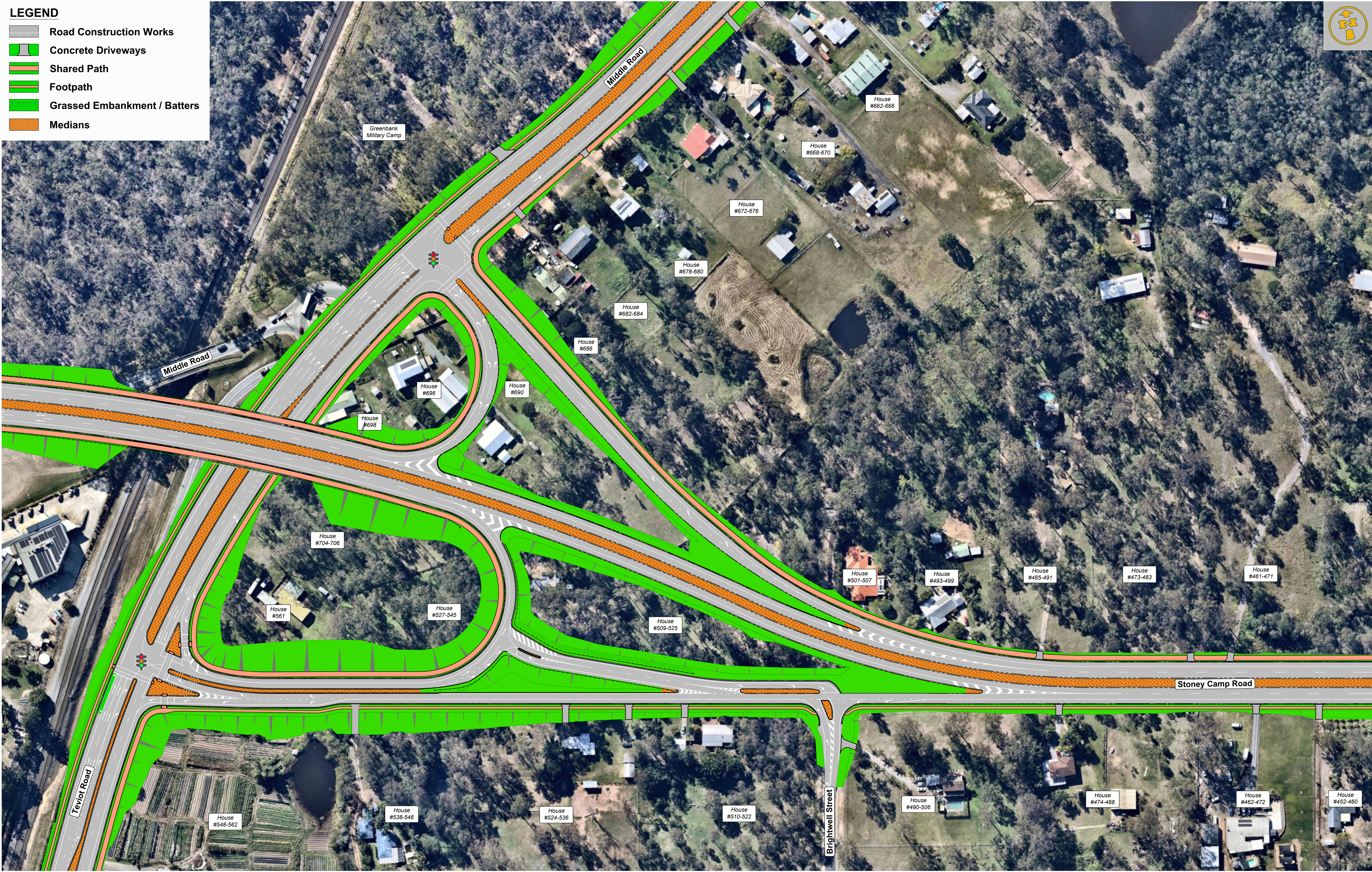
Teviot Road Upgrade, Greenbank Planning Concept Teviot Road / Middle Road Interchange Preliminary design | Indicative only
